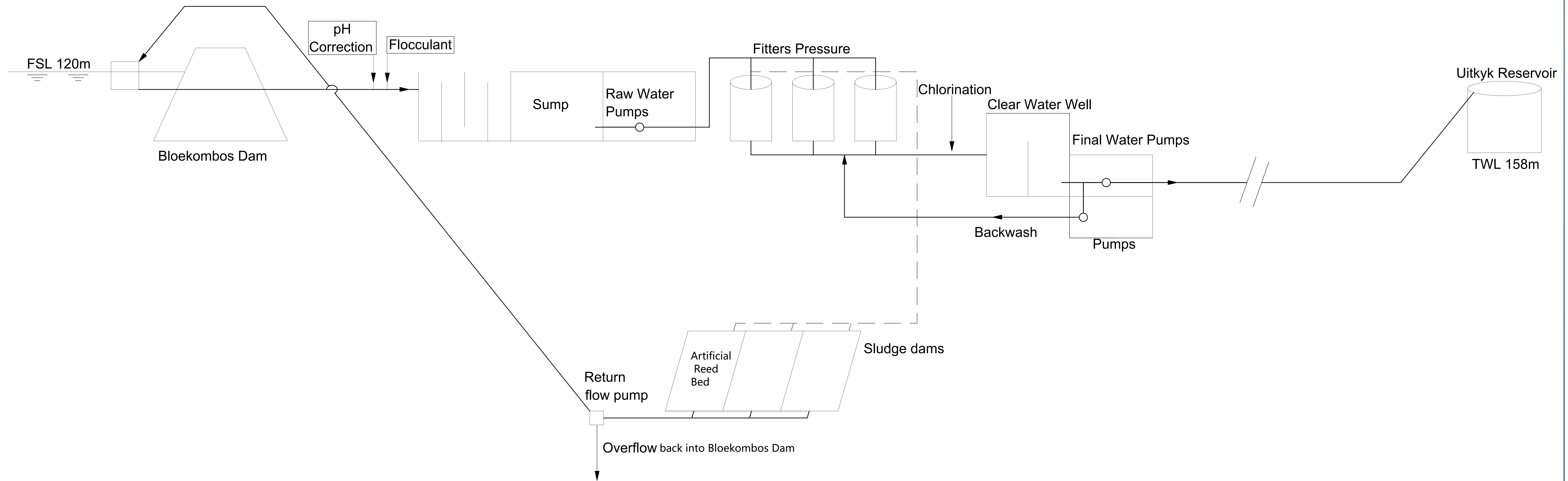
APPENDIX A: PROPOSED WTW PROCESS FLOW DIAGRAM
