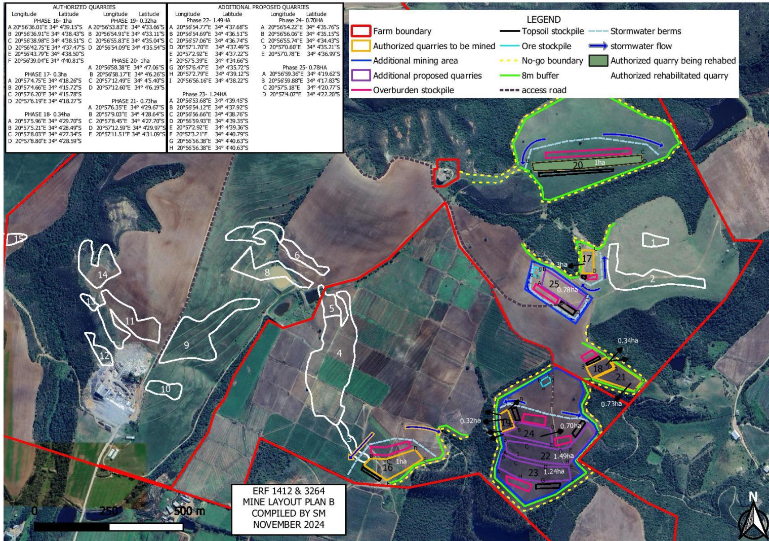
Fig 4: Proposed mining layout map for Erven RE/1412 and 3264 (previously Erf 1412) indicating approved mining right areas and proposed additional quarries.
